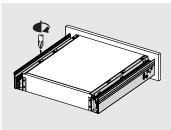
Fix screws
