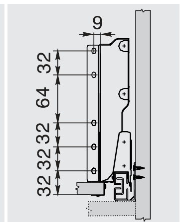
Back installation dimensions
