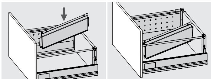
Side assembly
