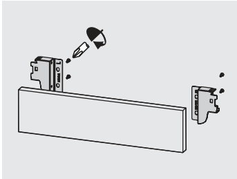
Back assembly
