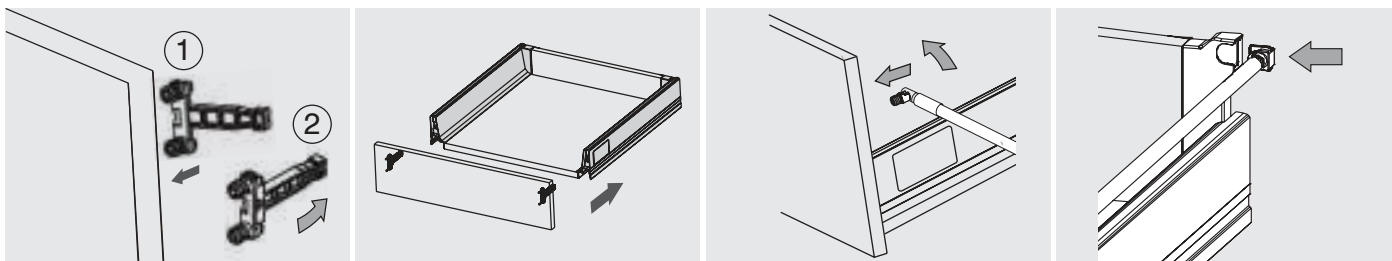
Front assembly
