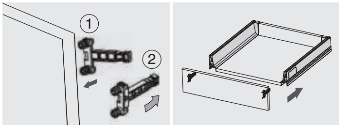
Front assembly
