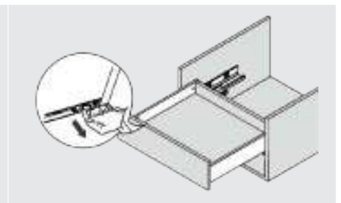
Press the locking device under the drawer bottom and pull out the drawer
