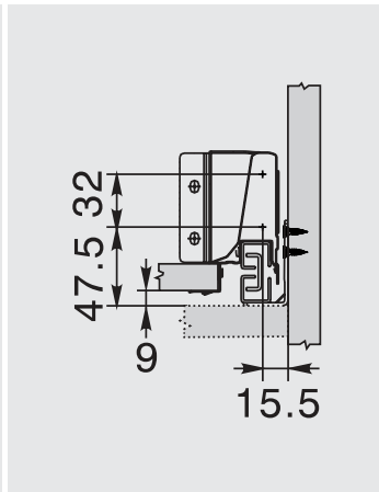
Front installation dimensions
