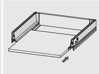
Bottom assembly
