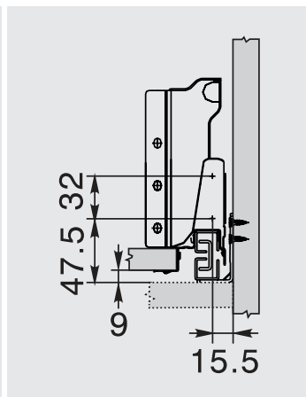
Front installation dimensions
