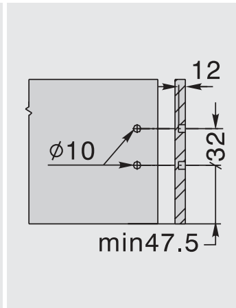
Front drilling dimensions
