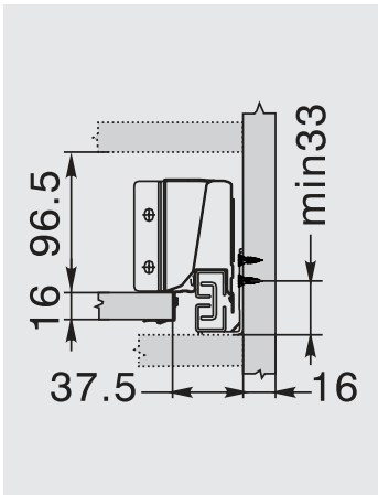
Space requirement in cabinet
